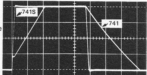
Response Comparison, SG741S vs. SG741, 10μS/div., 5V/div.
