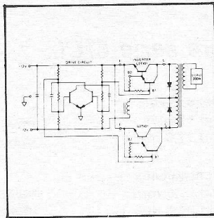
push-pull inverter
